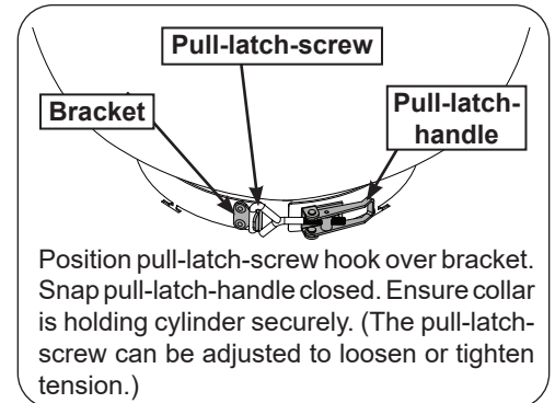
Fig. 3-2 Secure L.P. cylinder
