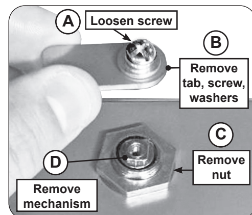
Fig. 2-5 Locking / unlocking
