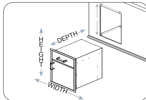
Fig. 4-1 Pantry cut-out diagram
