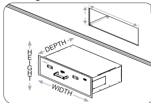
Fig. 4-5 Drawer cut-out diagram
