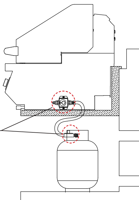
TYPICAL BOTTLE LP GAS HOOK-UP
