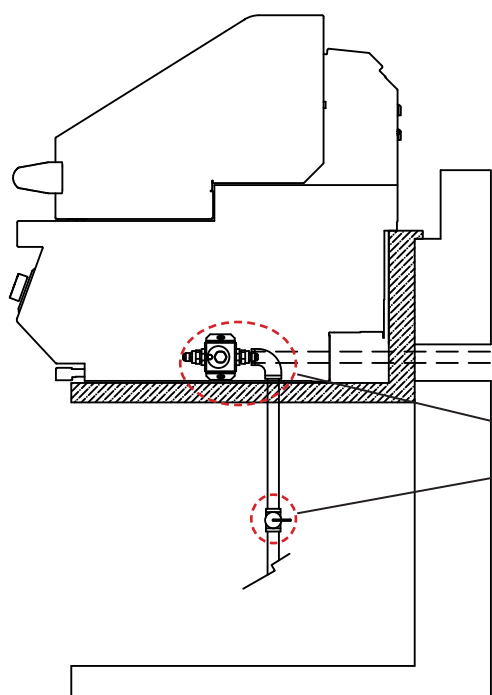
TYPICAL NATURAL GAS HOOK-UP
