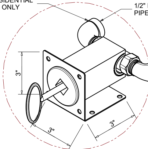
BRACKET DETAIL
