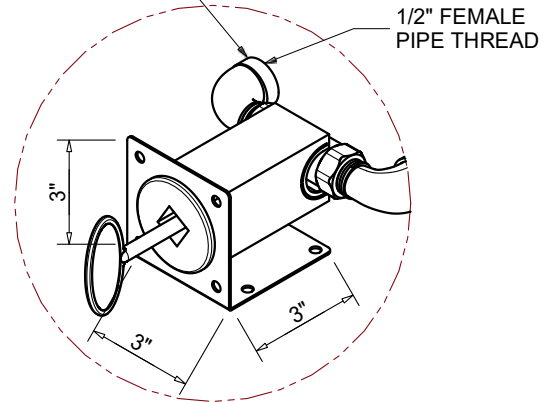
BRACKET DETAIL
