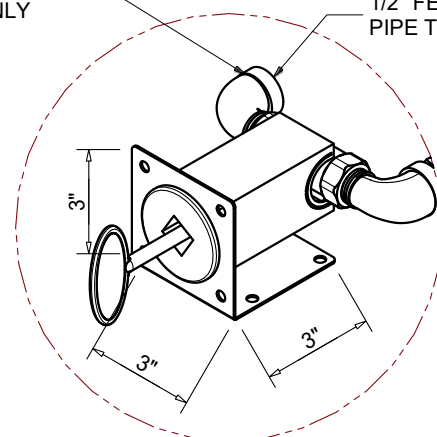
BRACKET DETAIL
