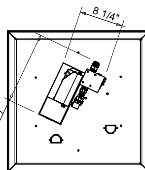
24SSEI-SQBL AND LARGER CONTROLS CONFIGURATION
