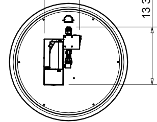
PENTA25EI AND LARGER CONTROLS CONFIGURATION
