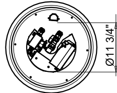
PENTA19EI AND 13SSEI CONTROLS CONFIGURATION
