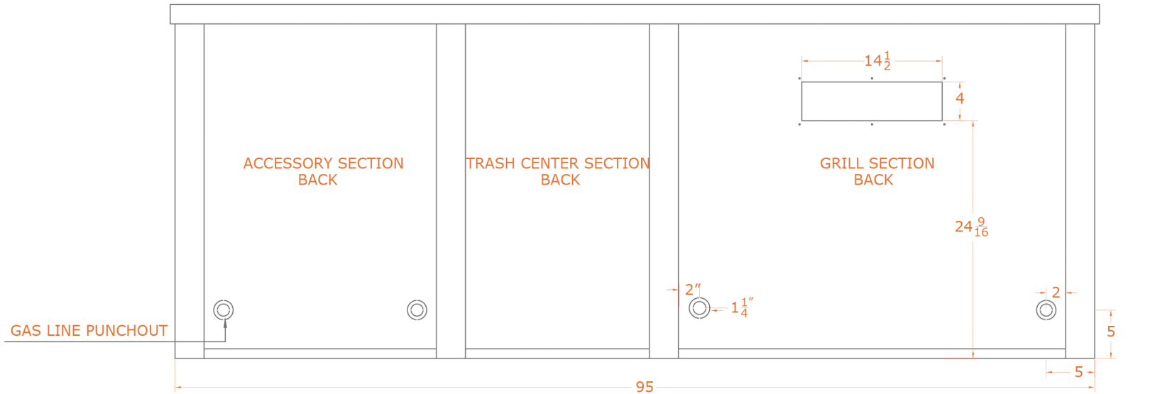
BACK VIEW
