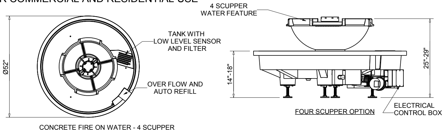
CONCRETE FIRE ON WATER - 4 SCUPPER
