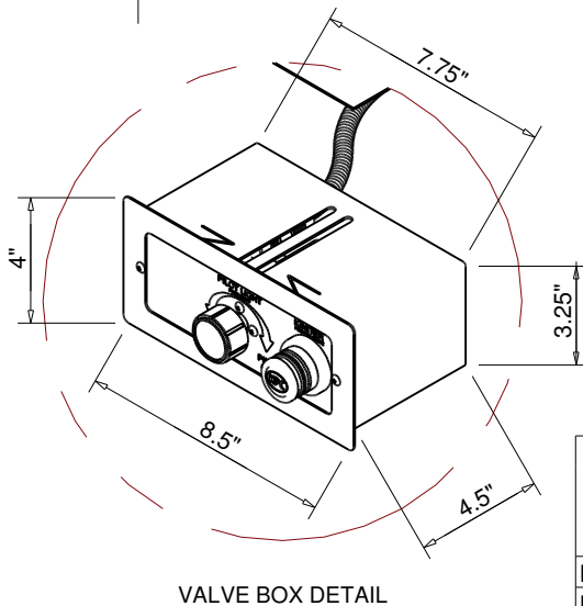
VALVE BOX DETAIL
