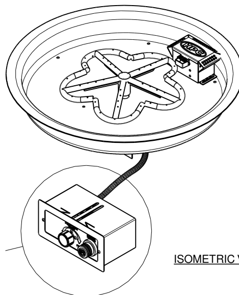
VALVE BOX DETAIL
