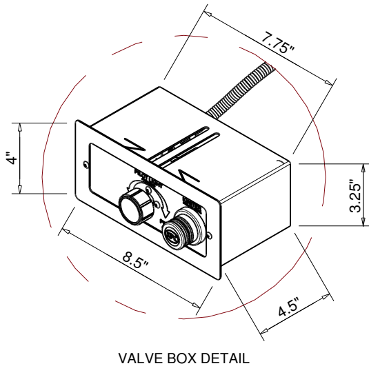
VALVE BOX DETAIL
