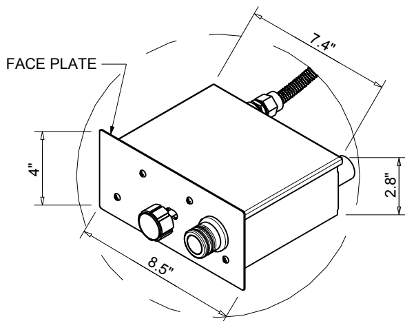
VALVE BOX DETAIL
