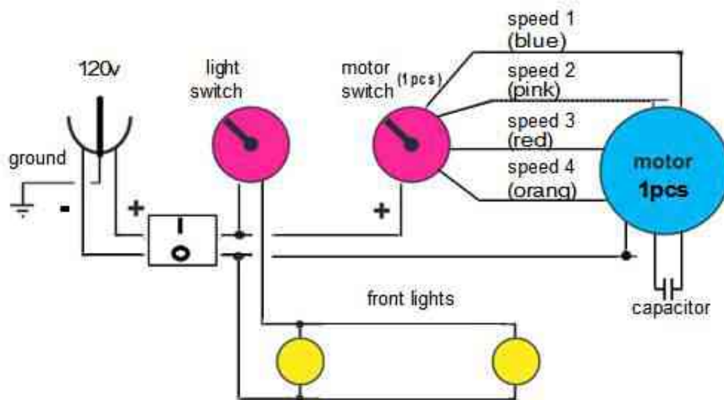
Wiring Diagram
