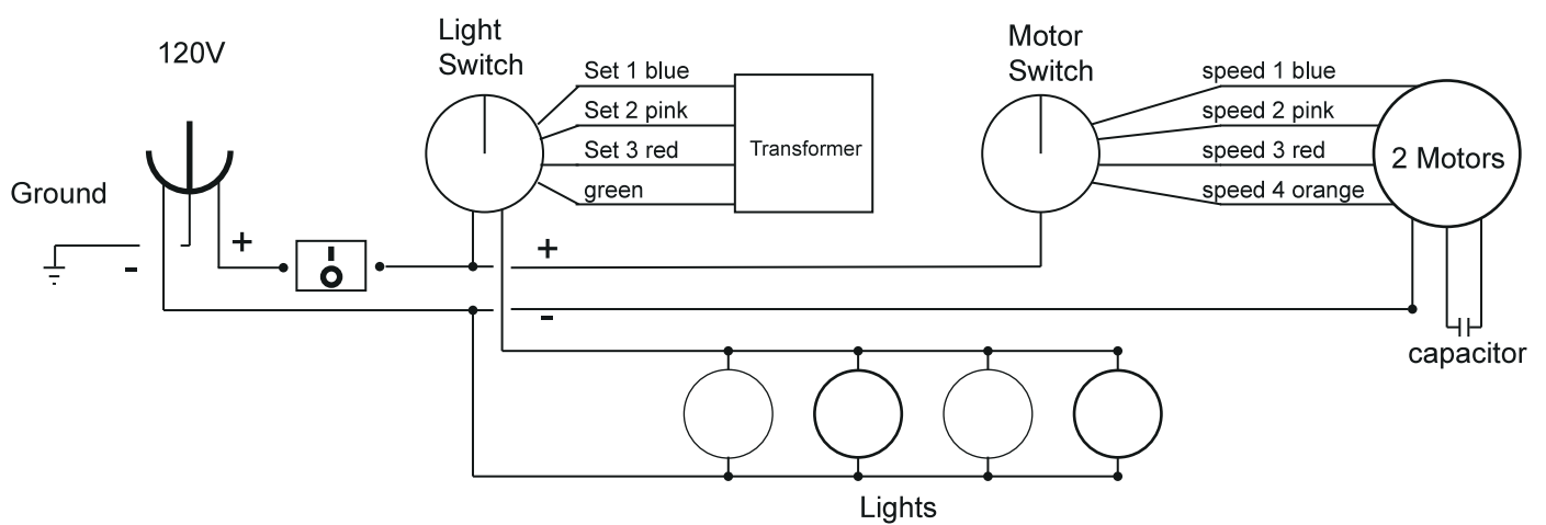
Wiring Diagram
