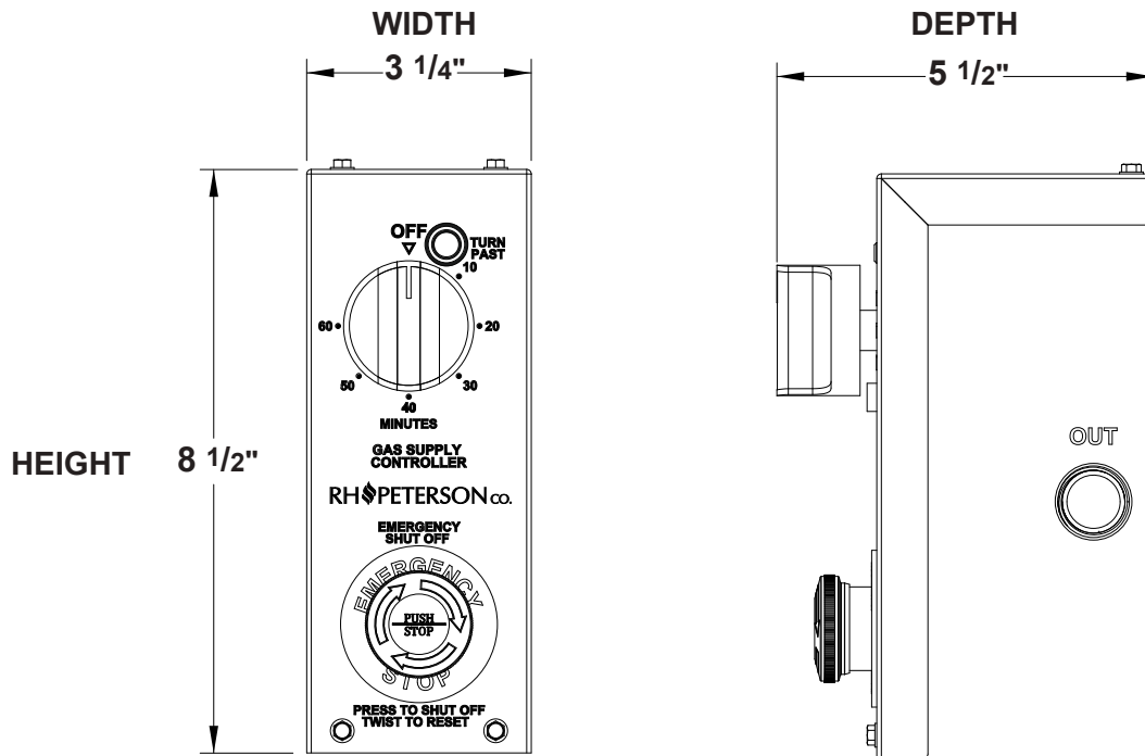
Fig. 2-1 Commercial dimensions
