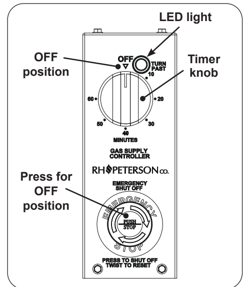
Fig. 5-1 Operation
