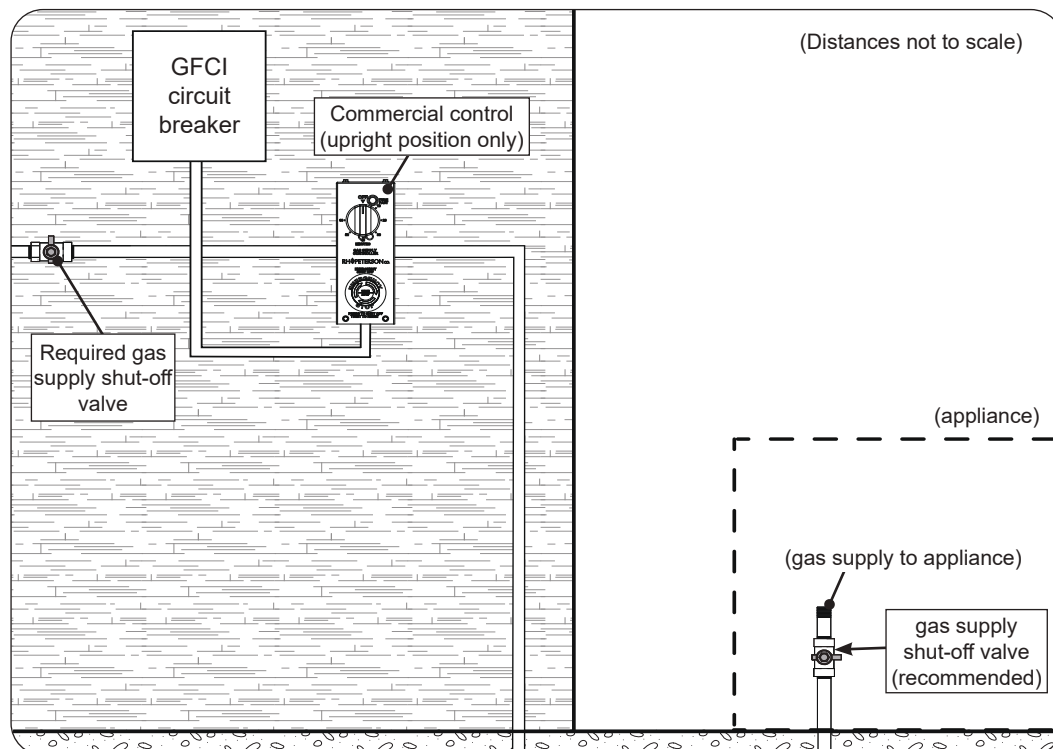
Fig. 2-2 Installation overview
