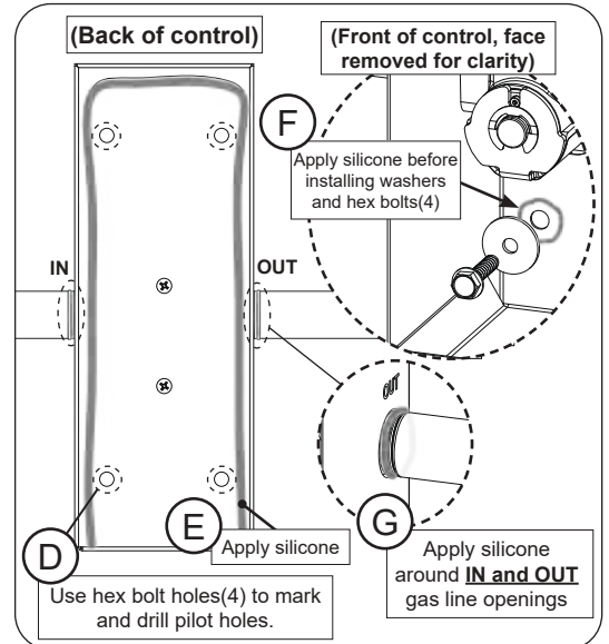
Fig. 4-2 Mount control
