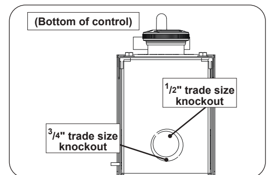
Fig. 4-3 Run electrical wiring
